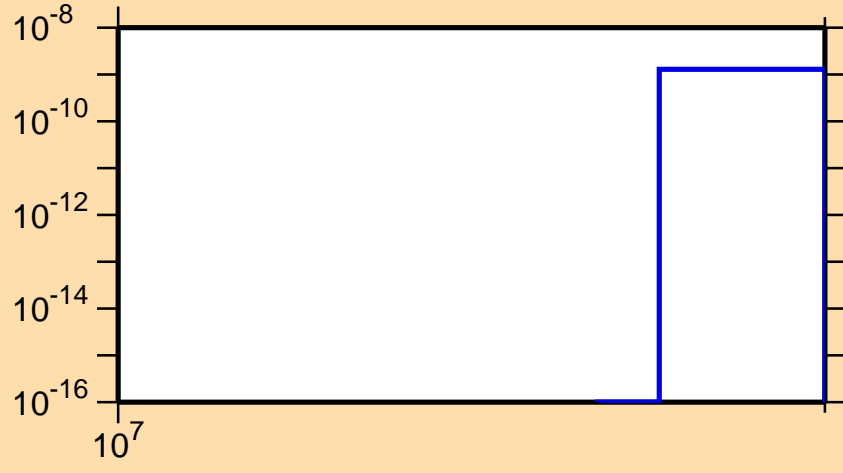
\sigma vs. E for ^{95}\text{Rh}(n,\text{pt})
