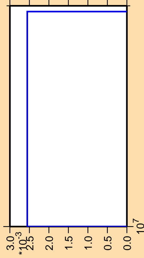
\Delta\sigma/\sigma vs. E for ^{95}\text{Rh} (mt 34)
