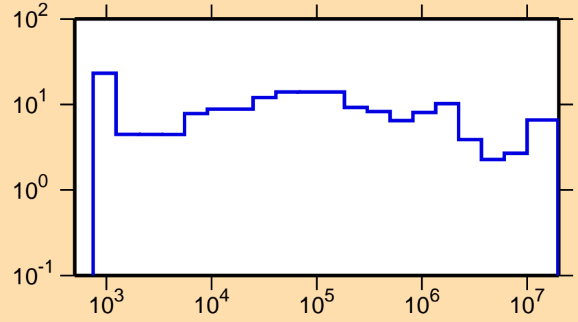
\Delta\sigma/\sigma vs. E for ^{95}\text{Rh}(n,\text{el.})
