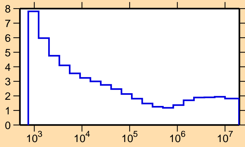
\sigma vs. E for ^{95}\text{Rh}(n,\text{nonel.})
