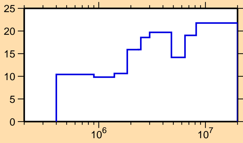
\Delta\sigma/\sigma vs. E for ^{95}\text{Rh}(n,n_1)
