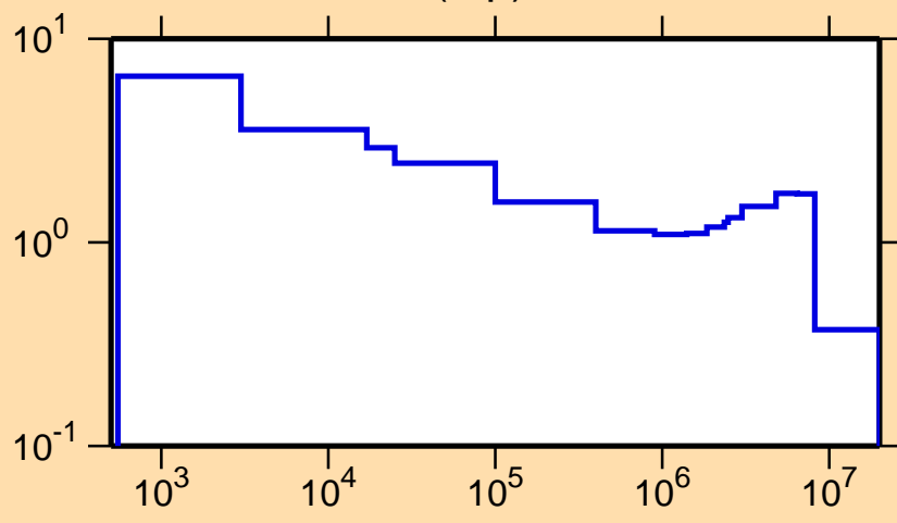
\sigma vs. E for ^{95}\text{Rh}(n,p)
