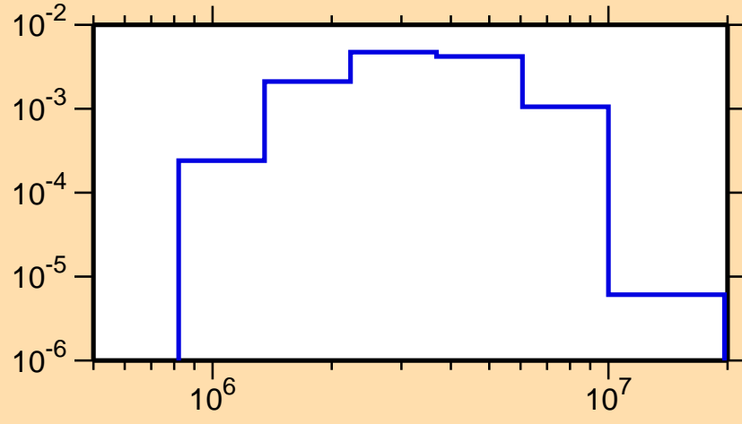
\sigma vs. E for ^{95}\text{Rh}(n,n_4)
