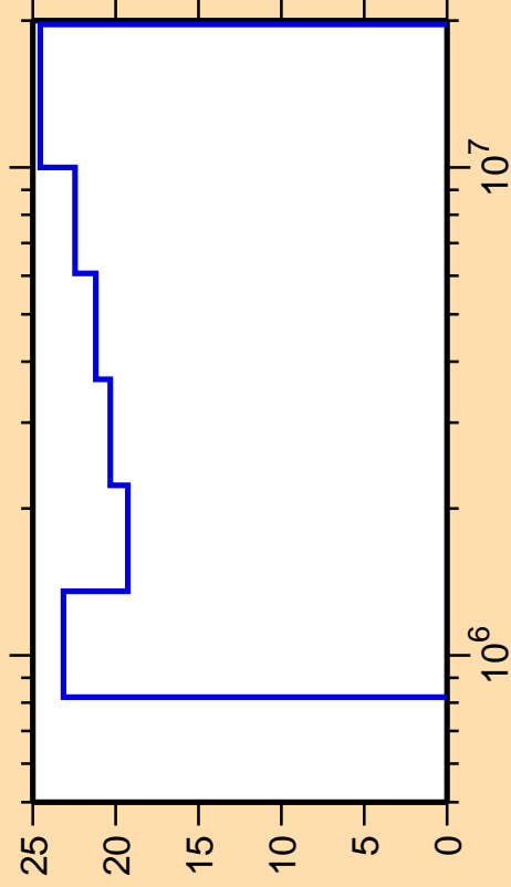
\Delta\sigma/\sigma vs. E for ^{95}\text{Rh}(n,n_4)
