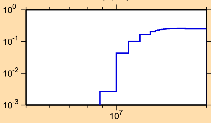
\sigma vs. E for ^{96}\text{Rh}(n,2n)
