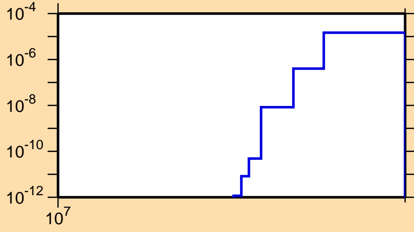
\sigma vs. E for ^{96}\text{Rh}(n,pt)
