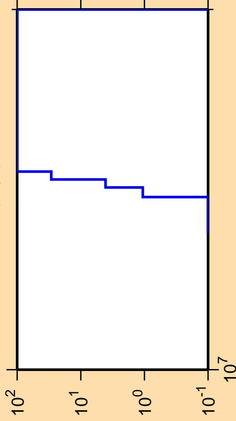
\Delta\sigma/\sigma vs. E for ^{96}\text{Rh}(n,pt)
