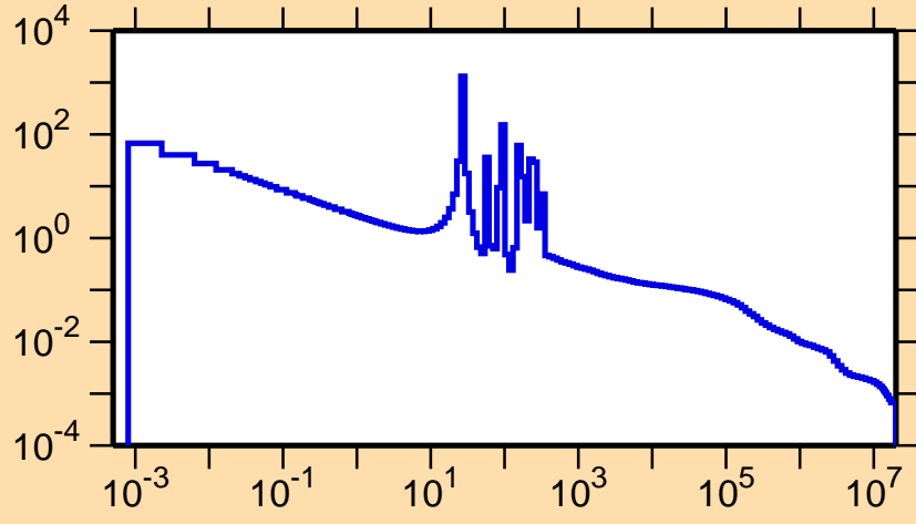
\sigma vs. E for ^{96}\text{Rh}(n,\gamma)
