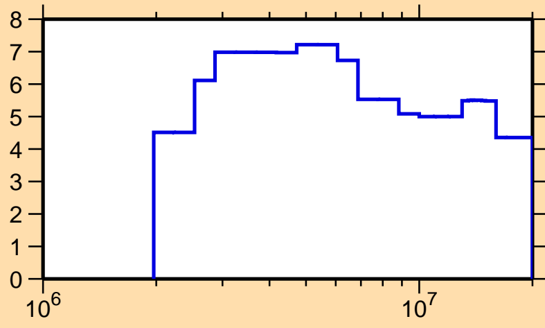
\Delta\sigma/\sigma vs. E for ^{96}\text{Rh}(n,n\text{nonel.})
