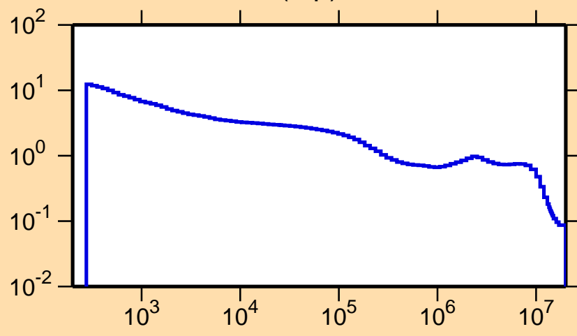
\sigma vs. E for ^{96}\text{Rh}(n,p)
