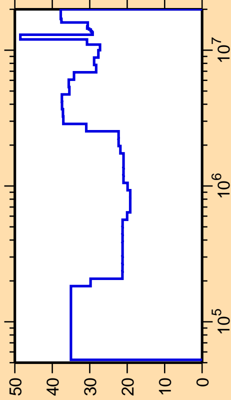
\Delta\sigma/\sigma vs. E for ^{96}\text{Rh}(n,n_1)
