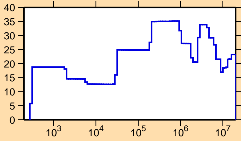
\Delta\sigma/\sigma vs. E for ^{96}\text{Rh}(n,p)
