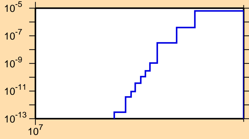
\sigma vs. E for ^{96}\text{Rh} (mt 45)
