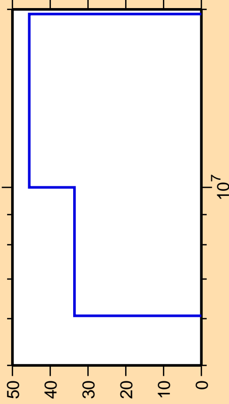
\Delta\sigma/\sigma vs. E for ^{96}\text{Rh}(n,n\alpha)
