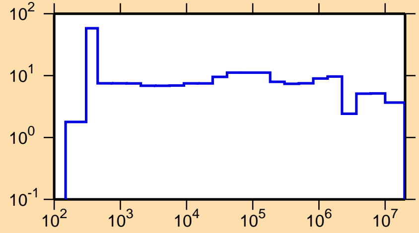
\Delta\sigma/\sigma vs. E for ^{96}\text{Rh}(n,\text{el.})
