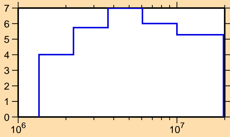
\Delta\sigma/\sigma vs. E for ^{96}\text{Rh}(n,n\text{onel.})
