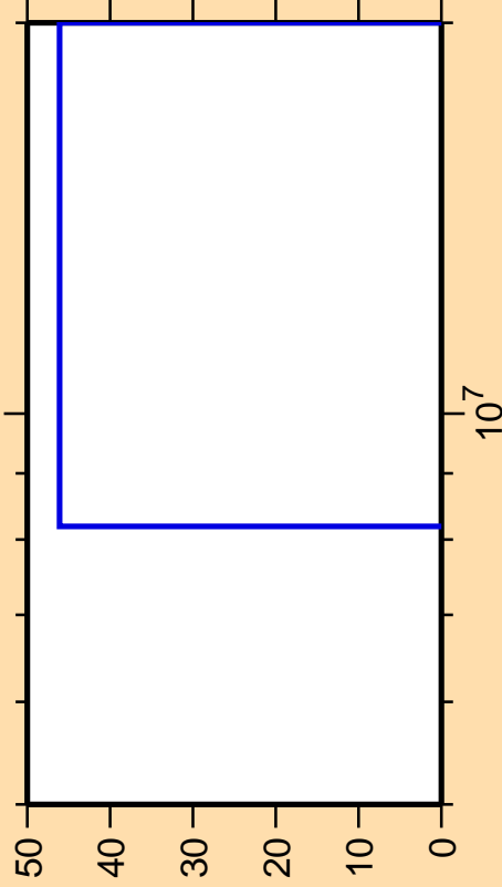
\Delta\sigma/\sigma vs. E for ^{96}\text{Rh}(\text{mt } 45)
