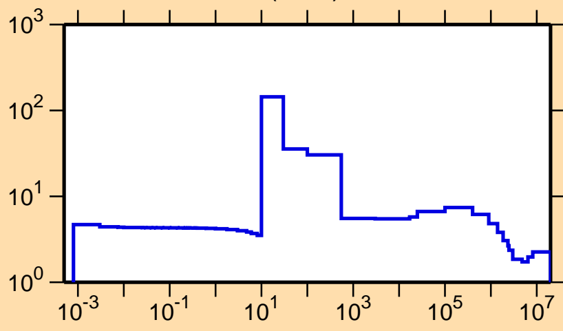
\sigma vs. E for ^{96}\text{Rh}(n,\text{el.})
