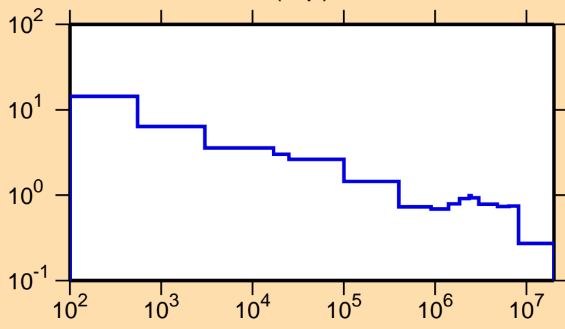
\sigma vs. E for ^{96}\text{Rh}(n,p)
