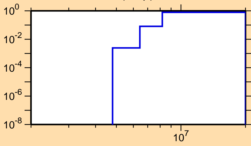
\sigma vs. E for ^{96}\text{Rh}(n,np)
