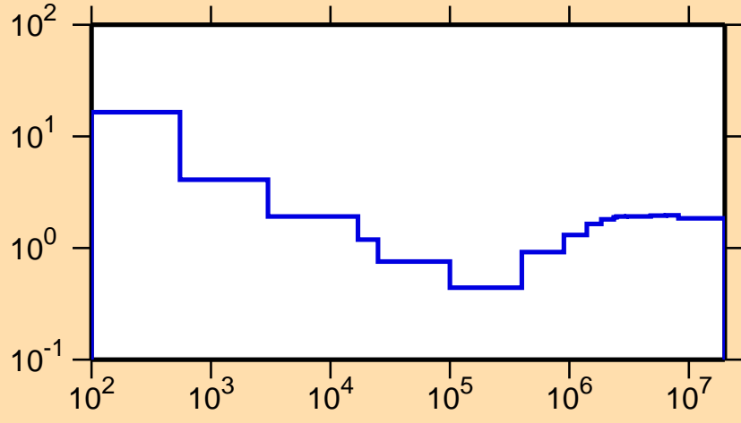
\sigma vs. E for ^{97}\text{Rh}(n,\text{nonel.})
