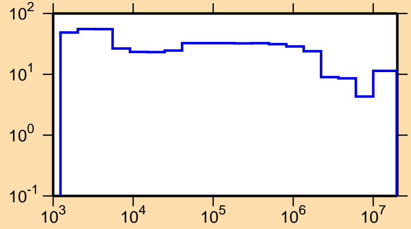
\Delta\sigma/\sigma vs. E for ^{97}\text{Rh}(n,\text{tot.})
