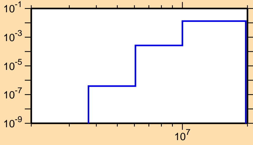
\sigma vs. E for ^{97}\text{Rh}(n,p\alpha)
