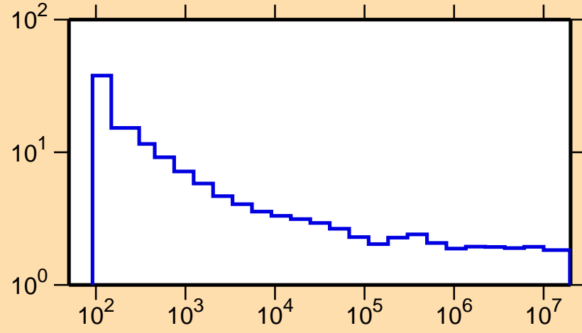
\sigma vs. E for ^{98}\text{Rh}(n,\text{nonel.})
