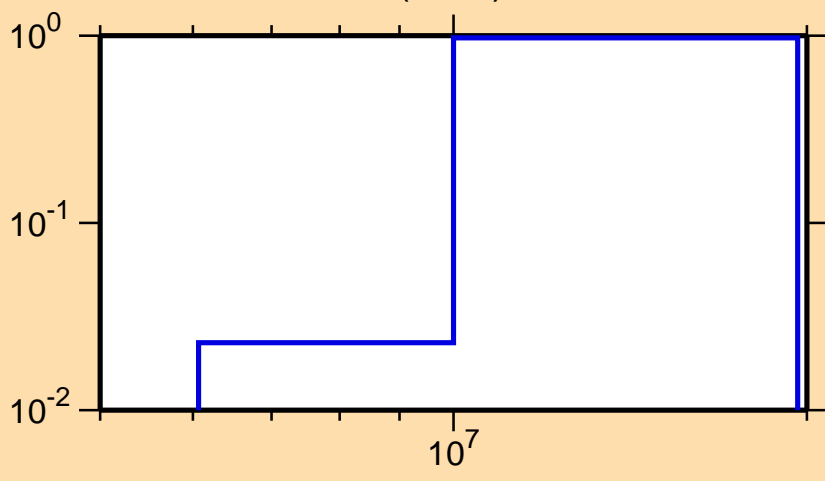
\sigma vs. E for ^{98}\text{Rh}(n,2n)
