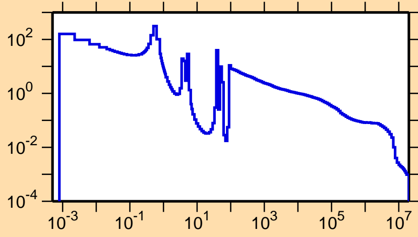
\sigma vs. E for ^{98}\text{Rh}(n,\gamma)
