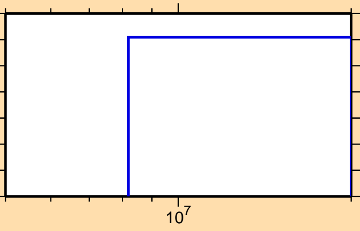
\sigma vs. E for ^{98}\text{Rh}(n,3n)
