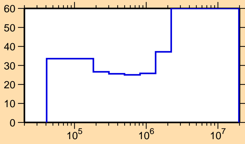
\Delta\sigma/\sigma vs. E for ^{99}\text{Rh}(n,n_1)
