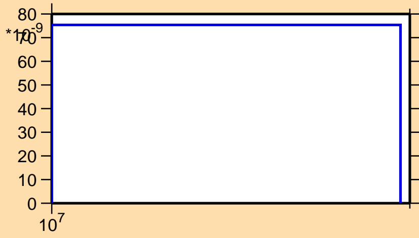
\sigma vs. E for ^{99}\text{Rh}(\text{mt } 45)
