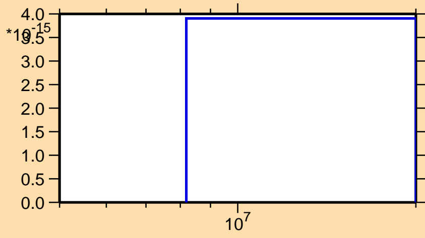
\sigma vs. E for ^{99}\text{Rh}(\text{mt } 34)
