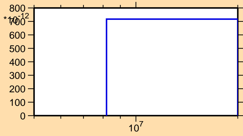
\sigma vs. E for ^{99}\text{Rh}(n,nt)
