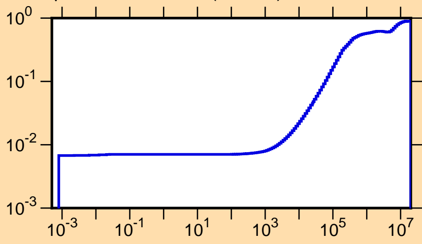
\mu vs. E for ^{100}\text{Rh}(\text{mt251})
