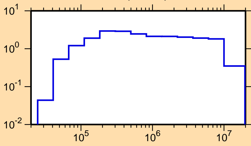
\sigma vs. E for ^{100}\text{Rh}(n,\text{inel.})
