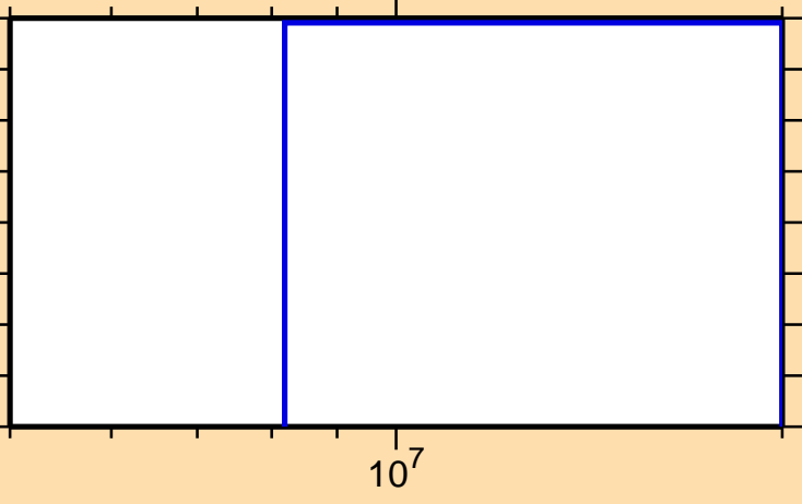
\sigma vs. E for ^{100}\text{Rh}(\text{mt117})
