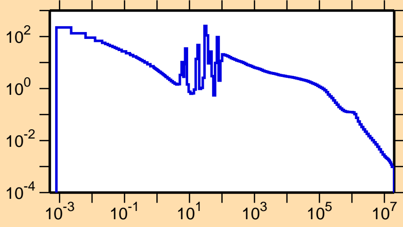
\sigma vs. E for ^{100}\text{Rh}(n,\gamma)
