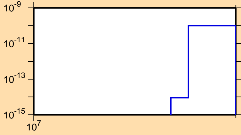
\sigma vs. E for ^{100}\text{Rh}(n,\text{pt})
