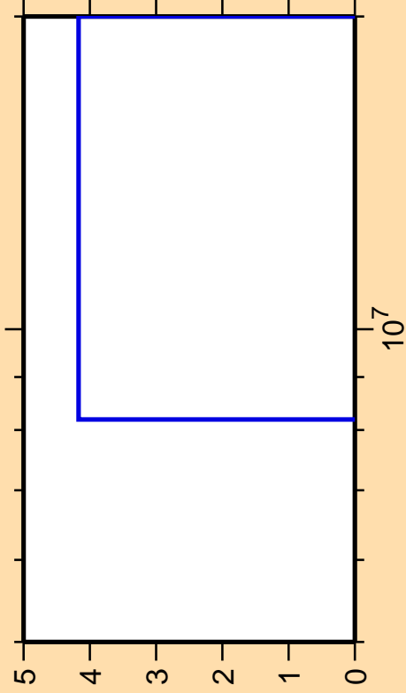
\Delta\sigma/\sigma vs. E for ^{100}\text{Rh}(n,\text{pt})
