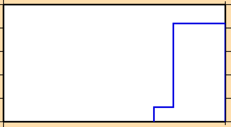
\sigma vs. E for ^{101}\text{Rh}(n,nt)
