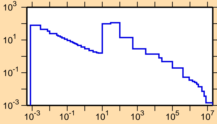
\sigma vs. E for ^{101}\text{Rh}(n,\gamma)
