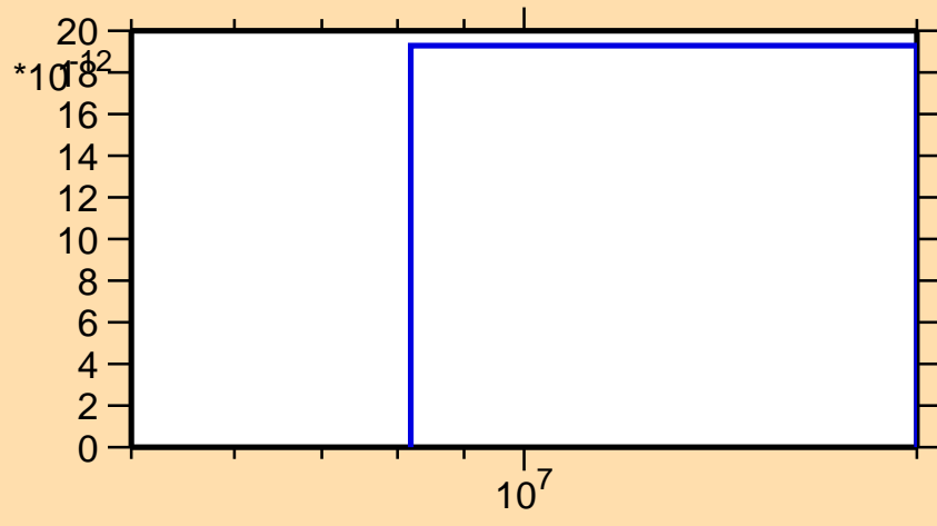
\sigma vs. E for ^{101}\text{Rh}(\text{mt } 45)
