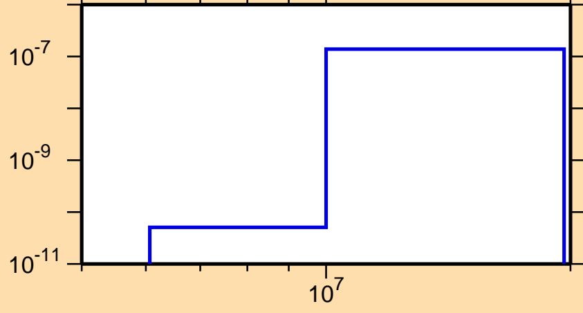
\sigma vs. E for ^{102}\text{Rh}(n,p\alpha)
