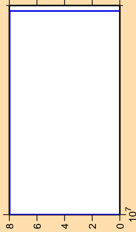
\Delta\sigma/\sigma vs. E for ^{102}\text{Rh}(\text{mt117})
