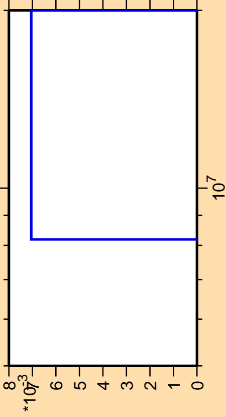
\Delta\sigma/\sigma vs. E for ^{102}\text{Rh}(\text{mt } 34)
