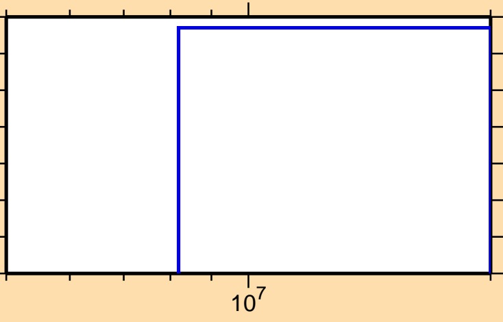
\sigma vs. E for ^{102}\text{Rh}(n,2n\alpha)
