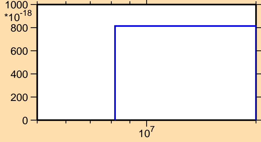
\sigma vs. E for ^{102}\text{Rh}(n,pd)
