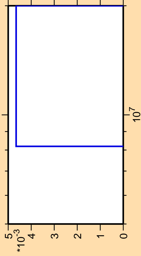
\Delta\sigma/\sigma vs. E for ^{102}\text{Rh}(n,pd)
