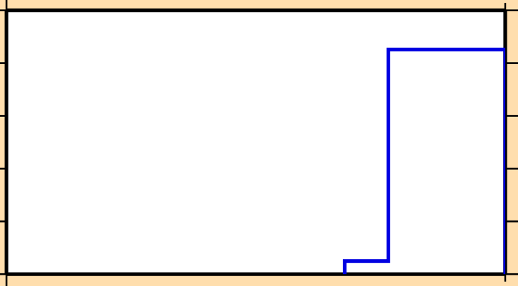
\sigma vs. E for ^{102}\text{Rh} (mt 34)
