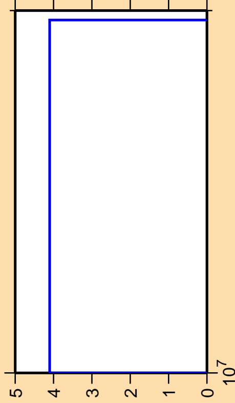
\Delta\sigma/\sigma vs. E for ^{102}\text{Rh} (mt 45)
