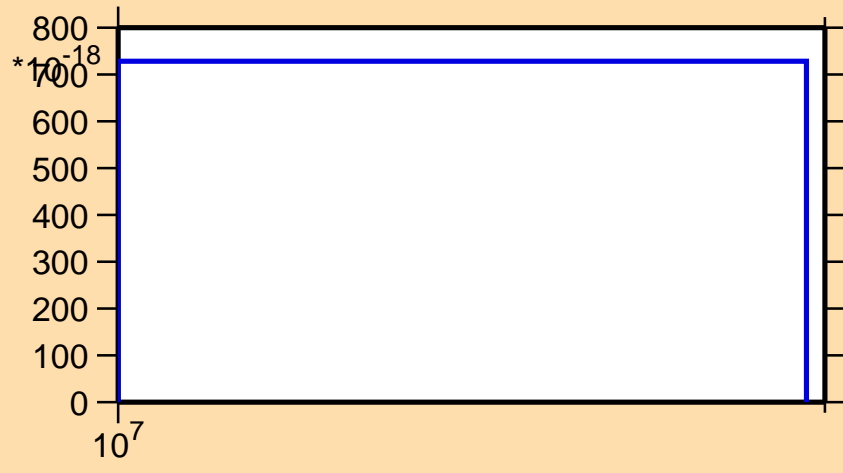
\sigma vs. E for ^{102}\text{Rh}(n,pd)
