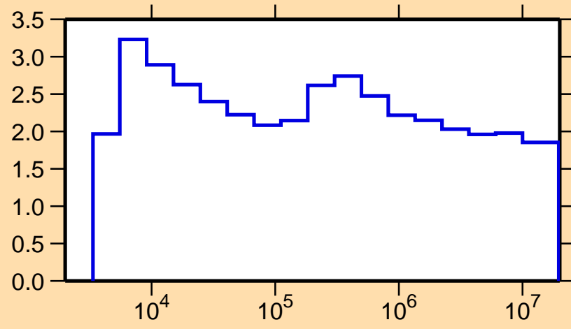
\sigma vs. E for ^{102}\text{Rh}(n,\text{nonel.})
