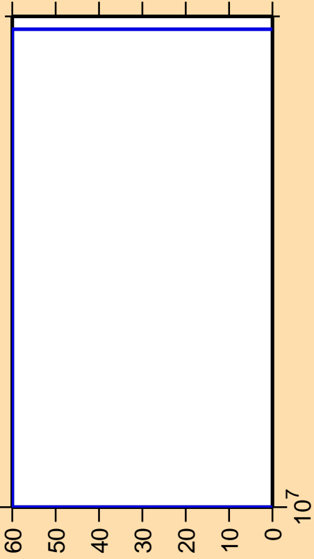
\Delta\sigma/\sigma vs. E for ^{103}\text{Rh}(n,2np)
