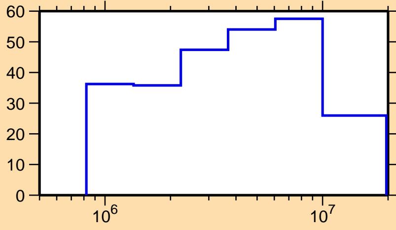
\Delta\sigma/\sigma vs. E for ^{103}\text{Rh}(n,p)
