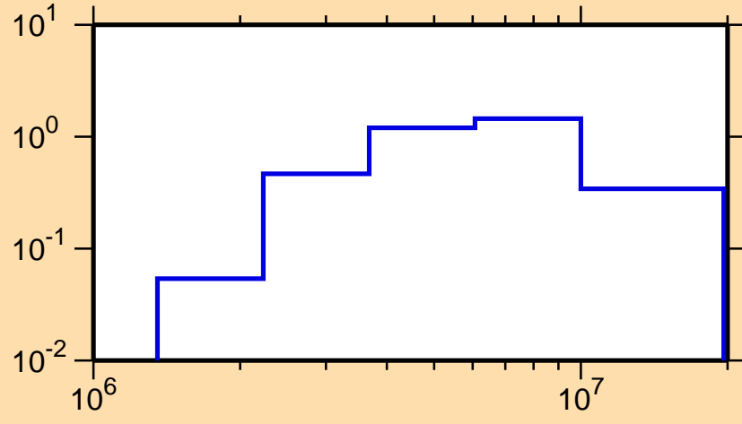
\sigma vs. E for ^{103}\text{Rh}(n,n\text{cont.})
