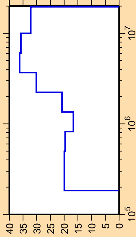
\Delta\sigma/\sigma vs. E for ^{103}\text{Rh}(n,n_3)
