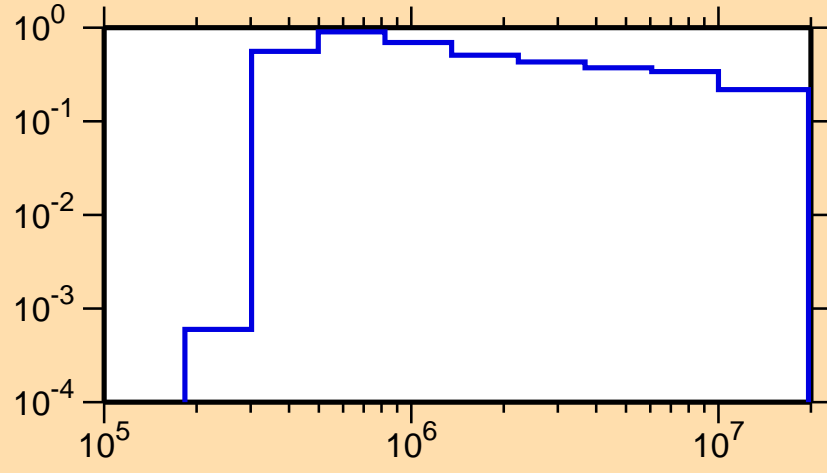
\sigma vs. E for ^{103}\text{Rh}(n,n_3)
