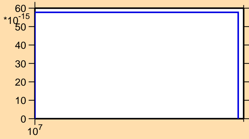
\sigma vs. E for ^{103}\text{Rh} (mt 45)
