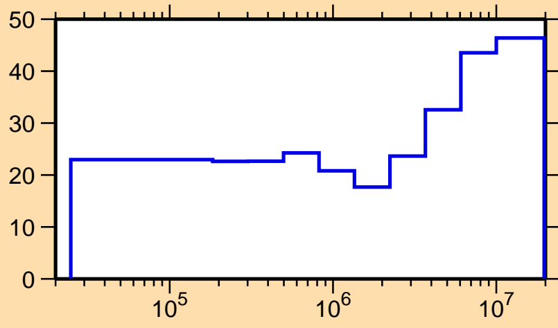
\Delta\sigma/\sigma vs. E for ^{103}\text{Rh}(n,n_1)
