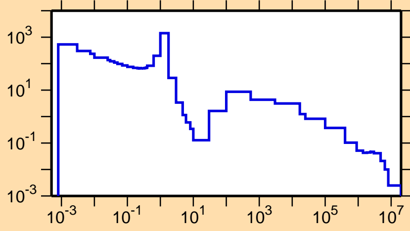
\sigma vs. E for ^{103}\text{Rh}(n,\gamma)
