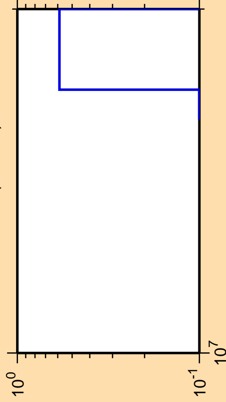
\Delta\sigma/\sigma vs. E for ^{104}\text{Rh}(\text{mt117})
