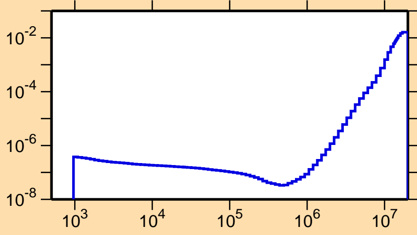
\sigma vs. E for ^{104}\text{Rh}(n,\alpha)
