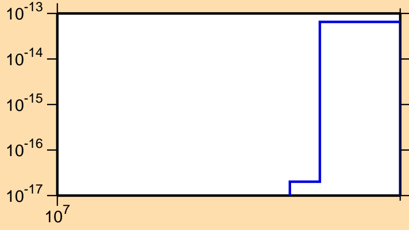
\sigma vs. E for ^{104}\text{Rh}(\text{mt117})
