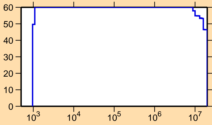
\Delta\sigma/\sigma vs. E for ^{104}\text{Rh}(n,p)
