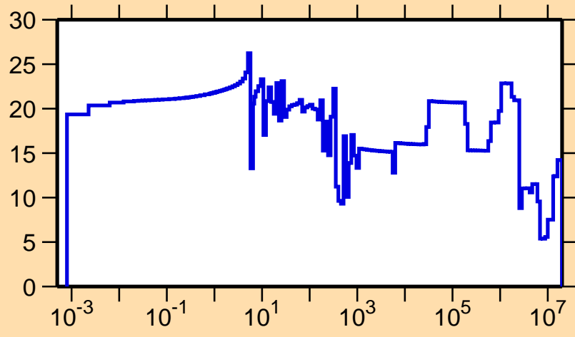
\Delta\sigma/\sigma vs. E for ^{104}\text{Rh}(n,\text{el.})
