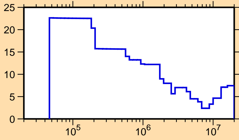
\Delta\sigma/\sigma vs. E for ^{104}\text{Rh}(n,\text{tot.})
