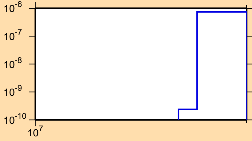
\sigma vs. E for ^{104}\text{Rh}(n,nt)
