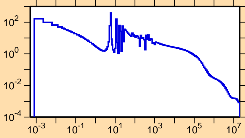
\sigma vs. E for ^{104}\text{Rh}(n,\gamma)
