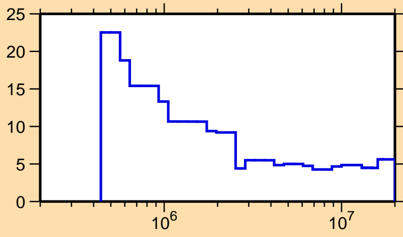
\Delta\sigma/\sigma vs. E for ^{104}\text{Rh}(n,\text{nonel.})
