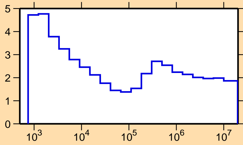
\sigma vs. E for ^{104}\text{Rh}(n,\text{nonel.})
