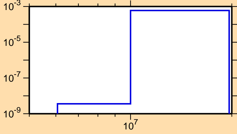
\sigma vs. E for ^{104}\text{Rh}(n,n\alpha)
