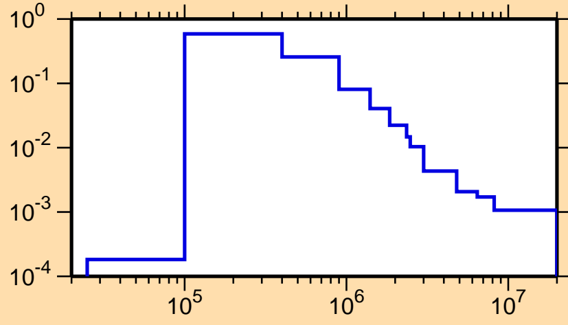
\sigma vs. E for ^{104}\text{Rh}(n,n_2)
