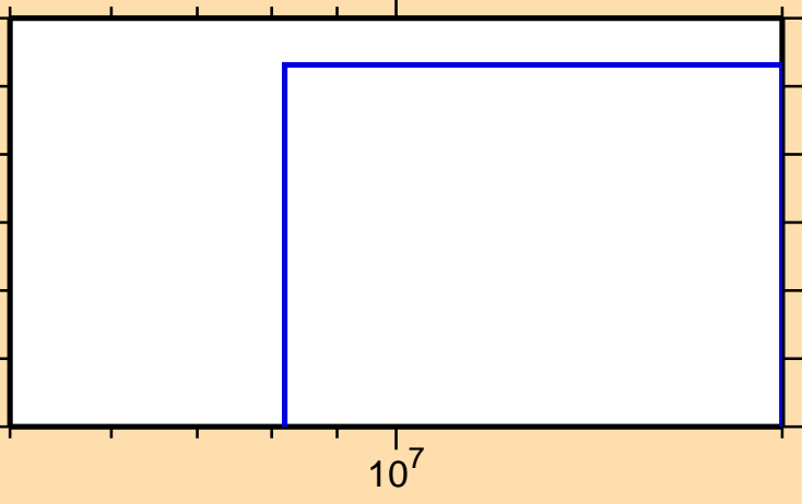
\sigma vs. E for ^{104}\text{Rh}(\text{mt117})
