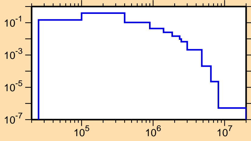
\sigma vs. E for ^{104}\text{Rh}(n,n_1)
