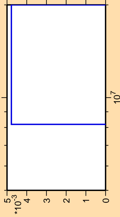
\Delta\sigma/\sigma vs. E for ^{104}\text{Rh}(\text{mt117})
