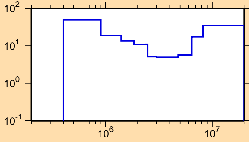
\Delta\sigma/\sigma vs. E for ^{104}\text{Rh}(n,n\text{cont.})
