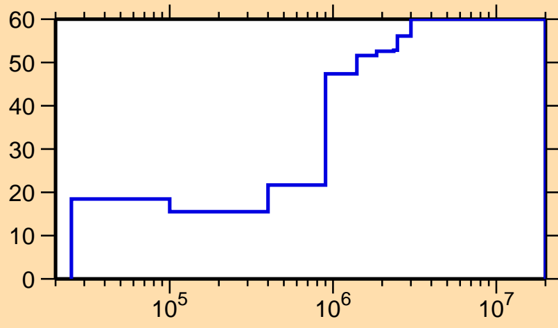
\Delta\sigma/\sigma vs. E for ^{104}\text{Rh}(n,n_1)
