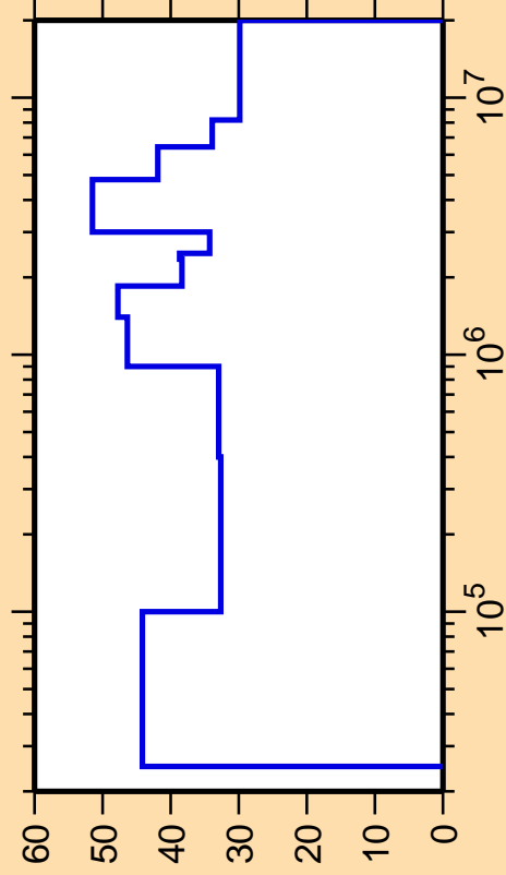
\Delta\sigma/\sigma vs. E for ^{104}\text{Rh}(n,n_2)
