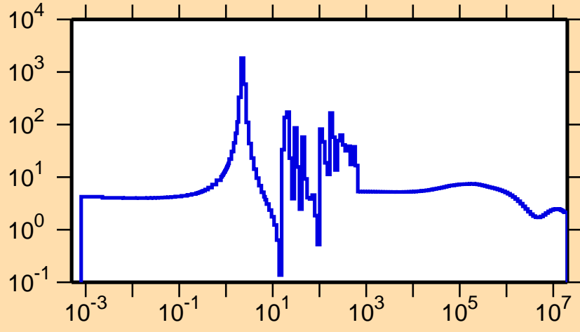
\sigma vs. E for ^{104}\text{Rh}(n,\text{el.})
