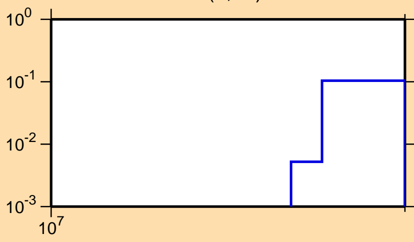
\sigma vs. E for ^{104}\text{Rh}(n,3n)
