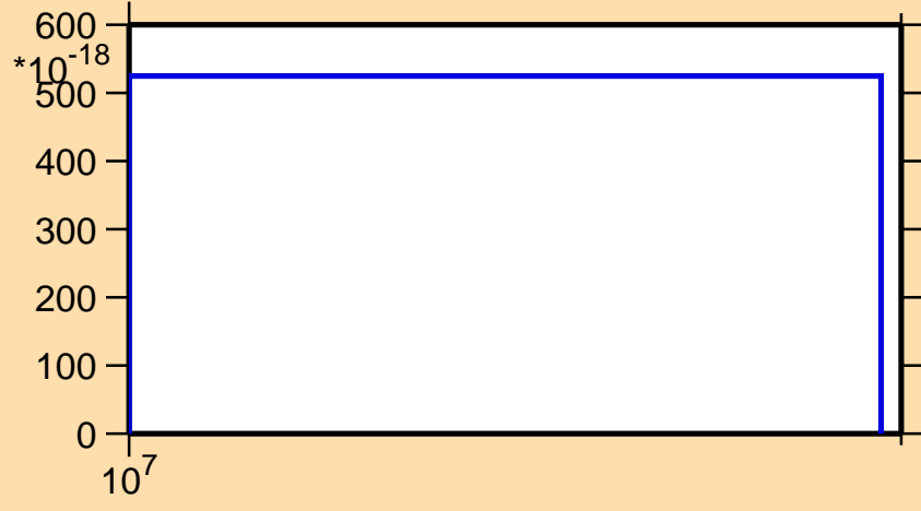
\sigma vs. E for ^{104}\text{Rh}(\text{mt117})
