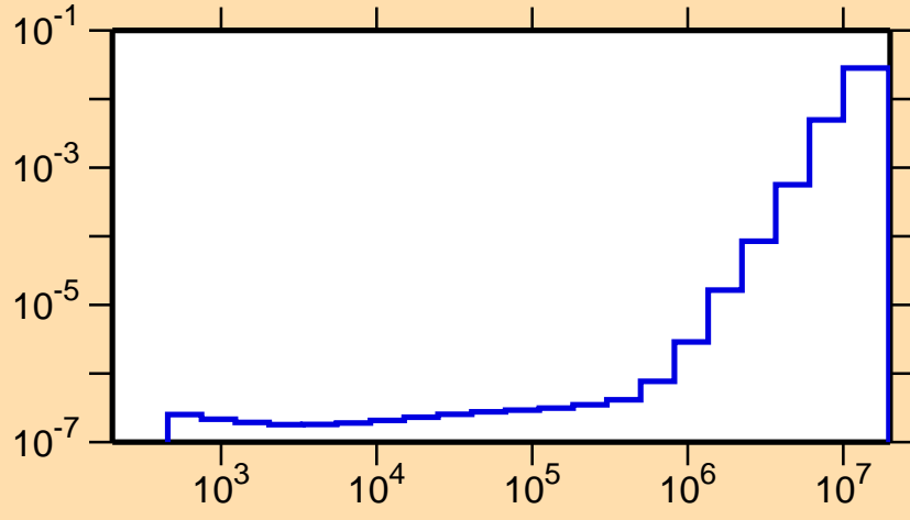
\sigma vs. E for ^{104}\text{Rh}(n,p)
