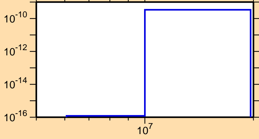
\sigma vs. E for ^{104}\text{Rh}(n,p\alpha)
