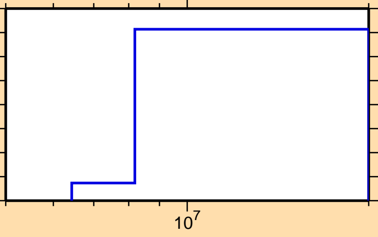
\sigma vs. E for ^{104}\text{Rh}(n,2n)
