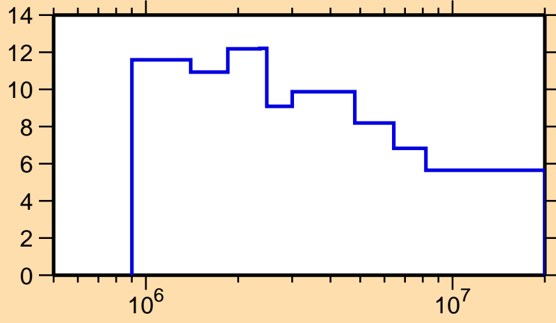
\Delta\sigma/\sigma vs. E for ^{105}\text{Rh}(n,n\text{nonel.})
