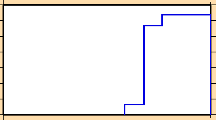
\sigma vs. E for ^{105}\text{Rh}(n,3n)
