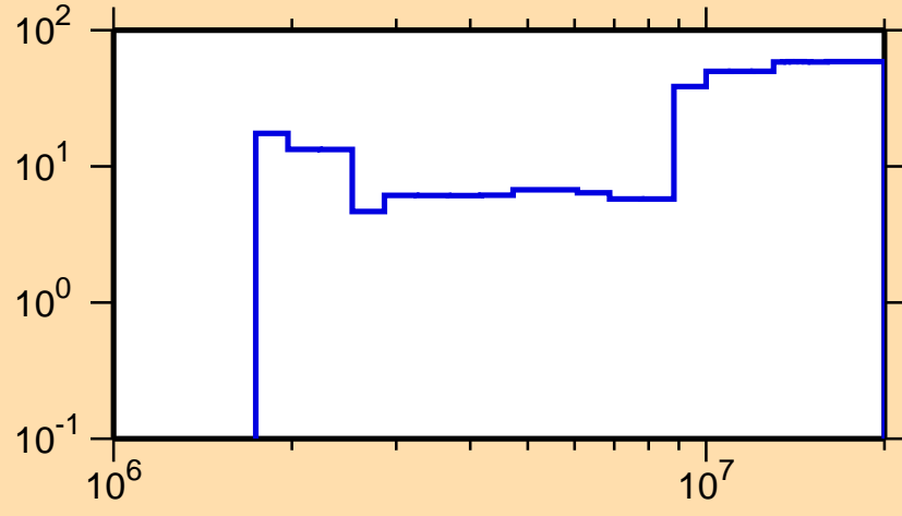
\Delta\sigma/\sigma vs. E for ^{105}\text{Rh}(n,n\text{cont.})
