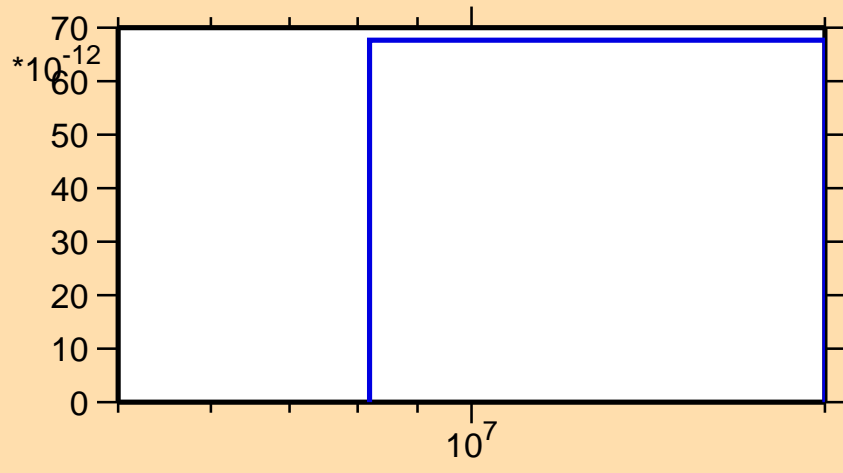
\sigma vs. E for ^{105}\text{Rh}(n,2n\alpha)
