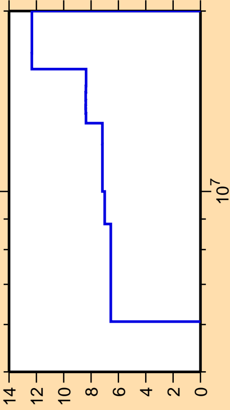
\Delta\sigma/\sigma vs. E for ^{106}\text{Rh}(n,2n)
