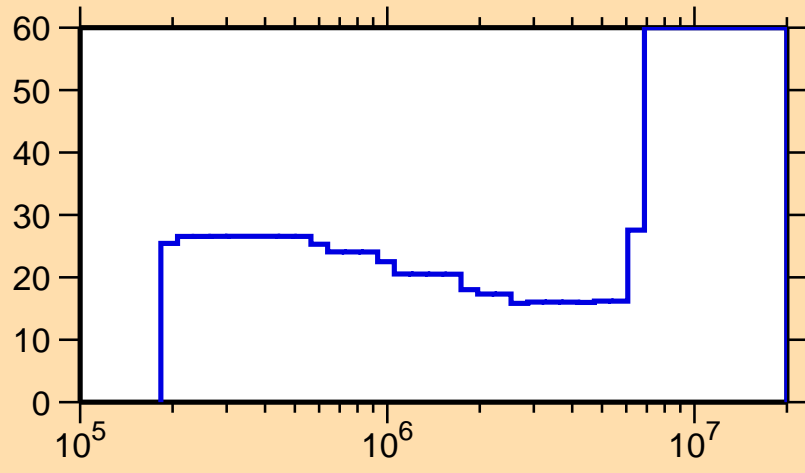
\Delta\sigma/\sigma vs. E for ^{106}\text{Rh}(n,\gamma)
