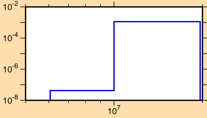
\sigma vs. E for ^{107}\text{Rh}(n,d)
