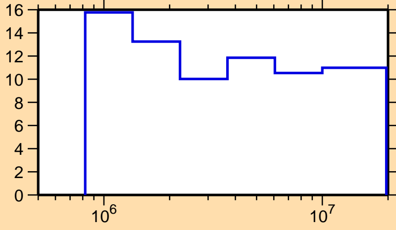
\Delta\sigma/\sigma vs. E for ^{107}\text{Rh}(n,n\text{onel.})
