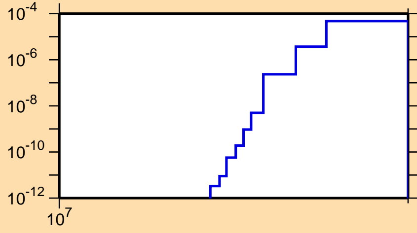
\sigma vs. E for ^{108}\text{Rh}(n,nd)
