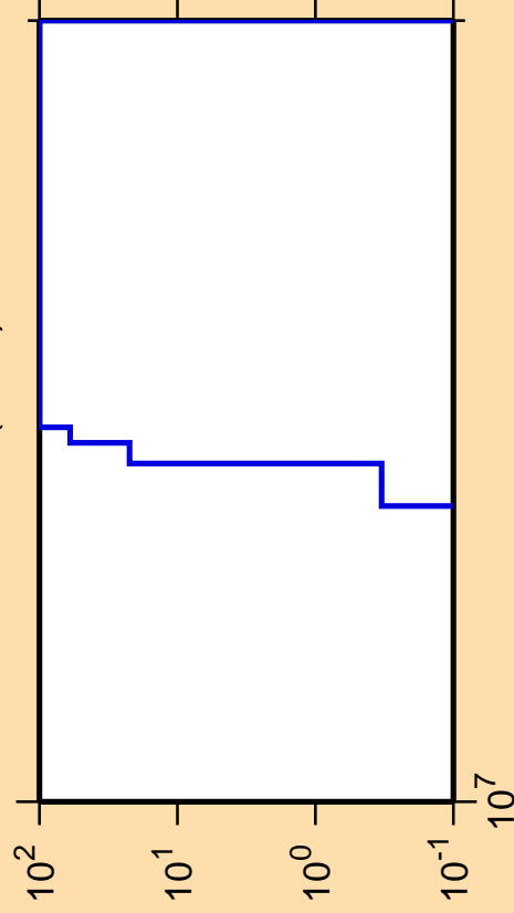
\Delta\sigma/\sigma vs. E for ^{108}\text{Rh}(n,nd)
