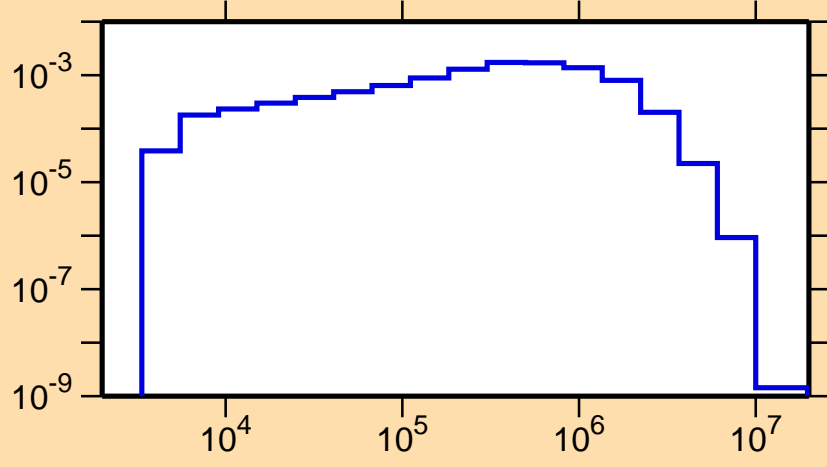
\sigma vs. E for ^{108}\text{Rh}(n,n_2)
