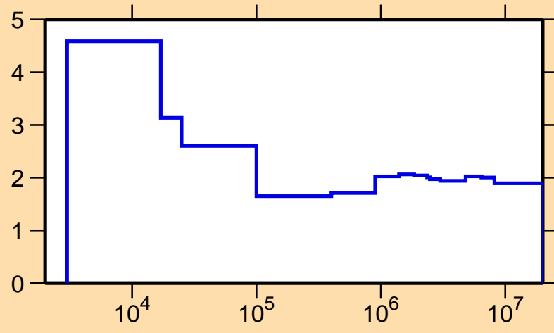
\sigma vs. E for ^{108}\text{Rh}(n,\text{nonel.})
