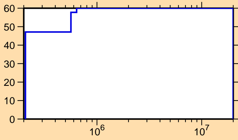
\Delta\sigma/\sigma vs. E for ^{109}\text{Rh}(n,n_1)
