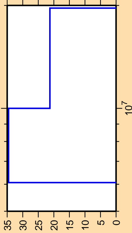
\Delta\sigma/\sigma vs. E for ^{109}\text{Rh}(n,2n)
