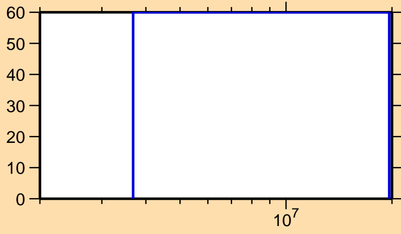
\Delta\sigma/\sigma vs. E for ^{109}\text{Rh}(n,p)
