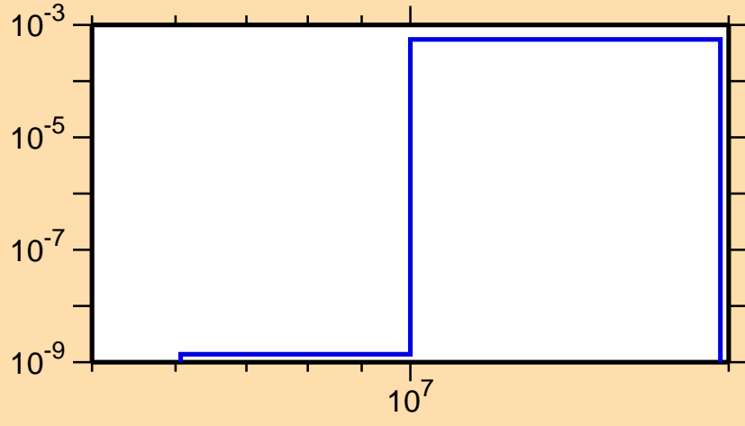
\sigma vs. E for ^{109}\text{Rh}(n,d)
