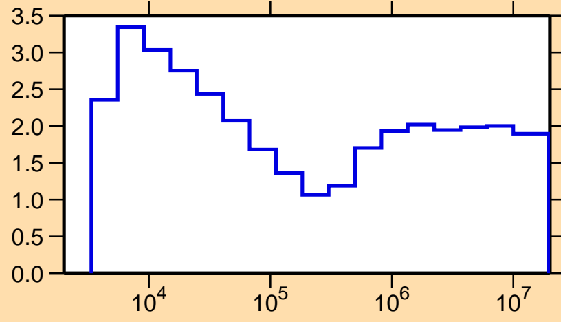
\sigma vs. E for ^{110}\text{Rh}(n,\text{nonel.})
