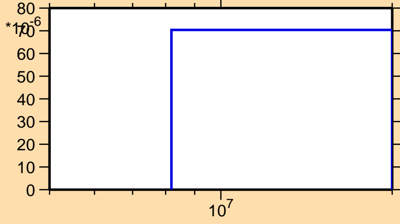
\sigma vs. E for ^{110}\text{Rh}(n,t)
