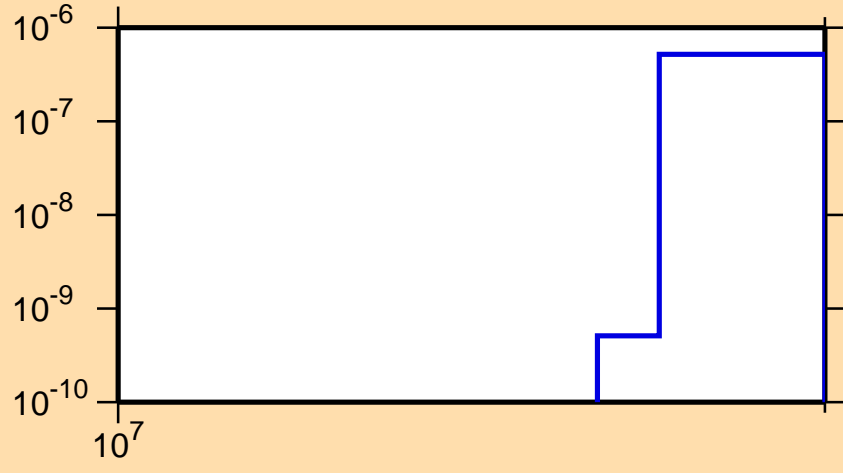
\sigma vs. E for ^{111}\text{Rh}(n,nt)
