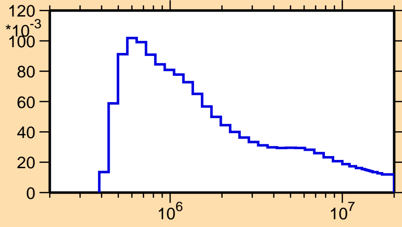
\sigma vs. E for ^{111}\text{Rh}(n,n_4)
