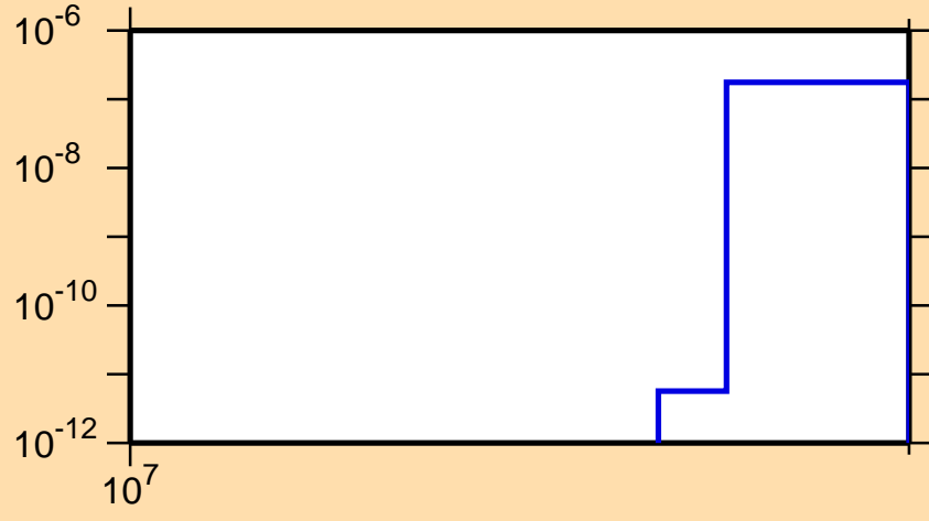
\sigma vs. E for ^{111}\text{Rh}(n,\text{nd})
