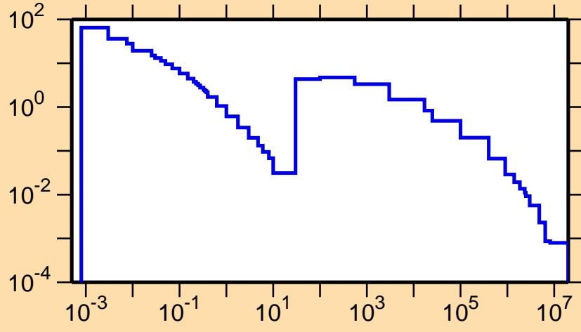
\sigma vs. E for ^{111}\text{Rh}(n,\gamma)
