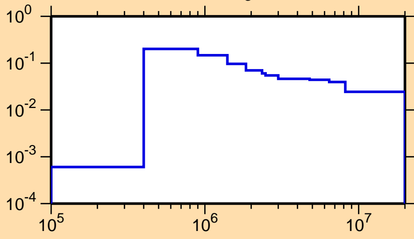
\sigma vs. E for ^{111}\text{Rh}(n,n_3)
