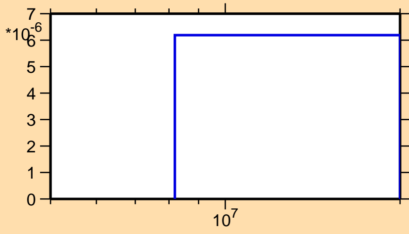
\sigma vs. E for ^{111}\text{Rh}(n,t)
