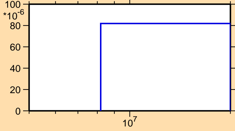
\sigma vs. E for ^{111}\text{Rh}(n,np)
