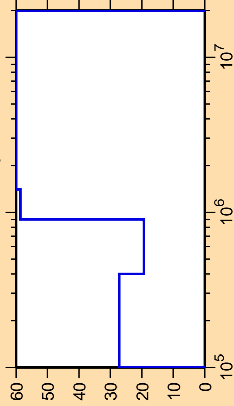
\Delta\sigma/\sigma vs. E for ^{111}\text{Rh}(n,n_3)
