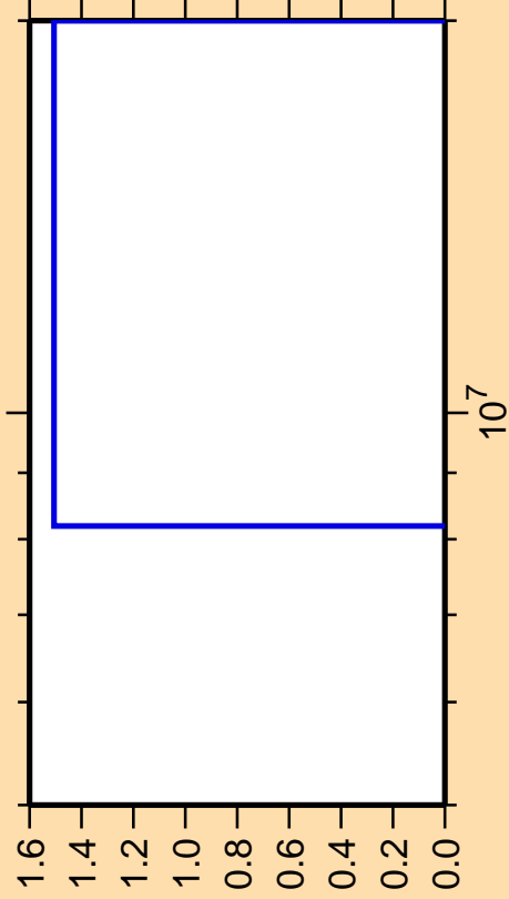
\Delta\sigma/\sigma vs. E for ^{111}\text{Rh}(n,2n\alpha)
