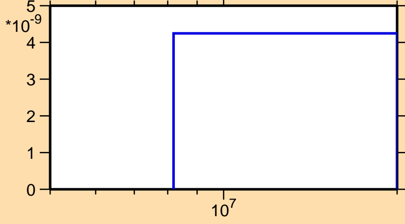
\sigma vs. E for ^{111}\text{Rh}(n,nt)
