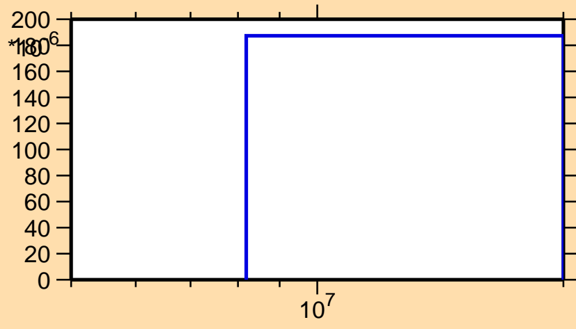
\sigma vs. E for ^{111}\text{Rh}(n,d)
