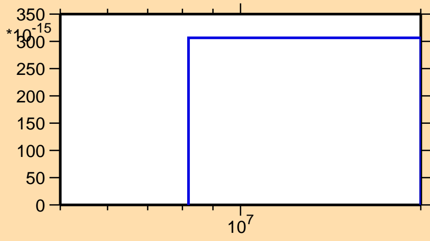
\sigma vs. E for ^{111}\text{Rh}(n,2n\alpha)
