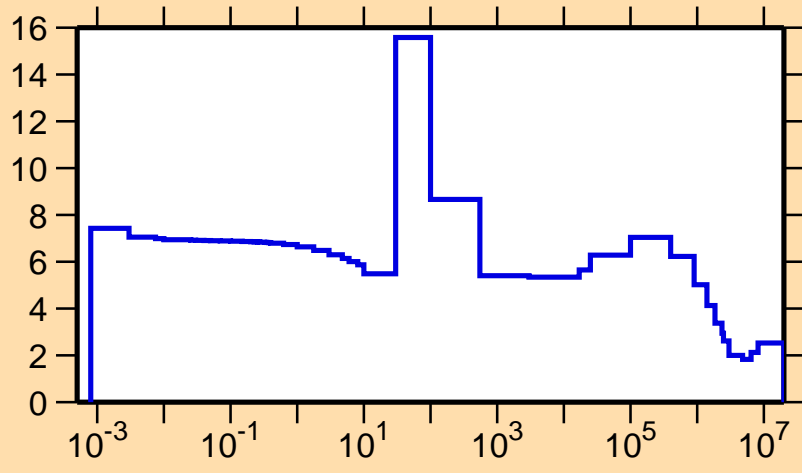
\sigma vs. E for ^{112}\text{Rh}(n,\text{el.})
