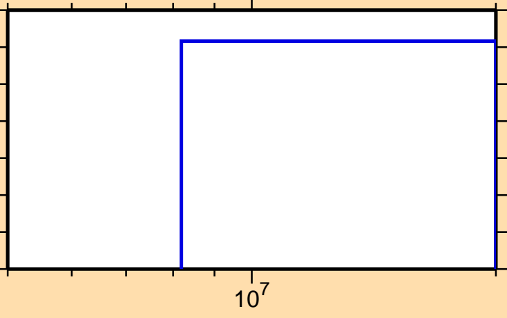
\sigma vs. E for ^{112}\text{Rh}(n,np)
