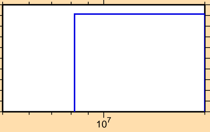
\sigma vs. E for ^{112}\text{Rh}(n,nt)
